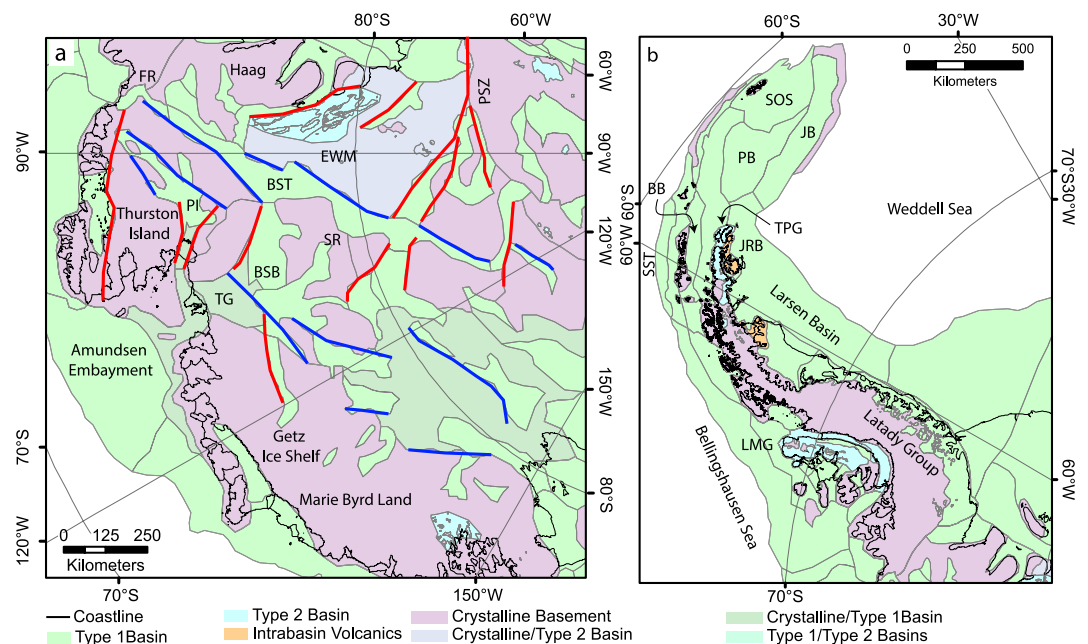
Figure 8. Sedimentary basins of the (a) Central West Antarctica and (b) Antarctic Peninsula Drake and eastern Weddell Sea regions. Structures in (a) are reinterpreted from prior studies (Bell et al., 1998; Bingham et al., 2012; Haeger & Kaban, 2019; T. A. Jordan et al., 2010b, 2013b, 2020; Studinger et al., 2001) as associated with the WARS (blue) and WSRS (red). PI, Pine Island Rift Basin; FR, Ferrigno Rift; BSB, Byrd Subglacial Basin; BST, Bentley Subglacial Trough; EWM, Ellsworth-Whitmore Mountains; SR, Sinuous Ridge; PSZ, Pagano Shear Zone; SST, South Shetland Trench; BB, Bransfield Basin; PB, Powell Basin; JB, Jane Basin; SOS, South Orkney Shelf; TPG, Trinity Peninsula Group; LMG, LeMay Group; JRB, James Ross Basin.
